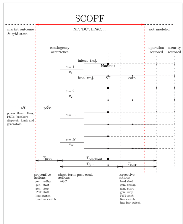
Illustration of calculation core supporting comparison of reliability criteria
