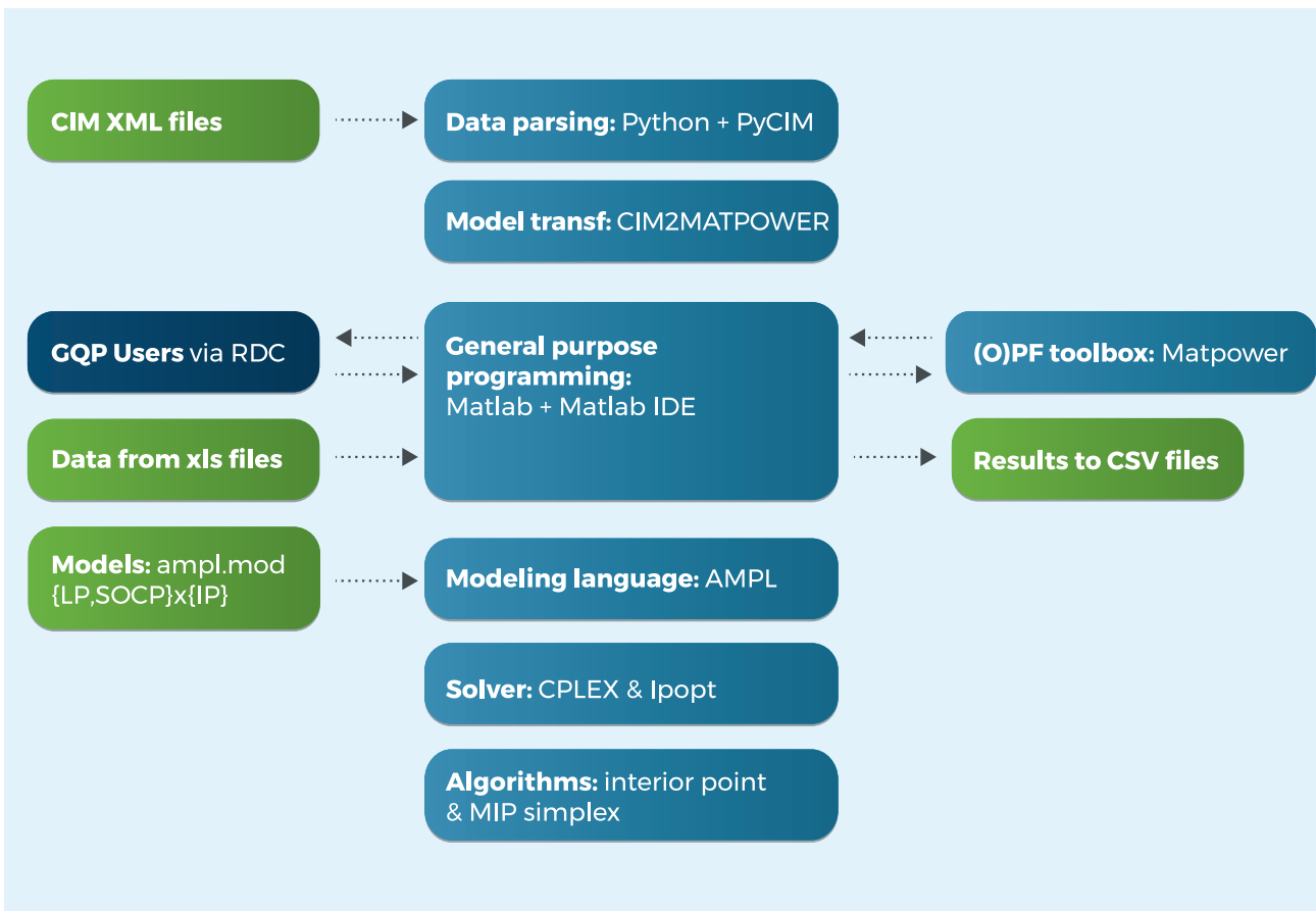
Illustration of calculation core supporting comparison of reliability criteria
