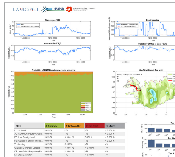
Web-based GUI for live risk outputs developed for the Landsnet pilot test
