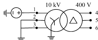
Fig. 14. Excitation on high-voltage side.
