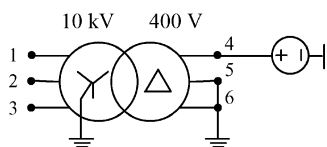
Fig. 20. Excitation on low-voltage side.
