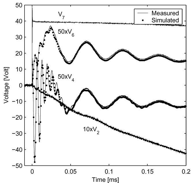
Fig. 17. Voltage responses.
