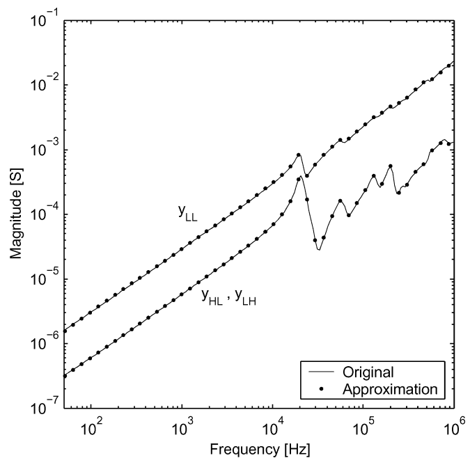
Fig. 10. Rational approximation of measured zero sequence system.
